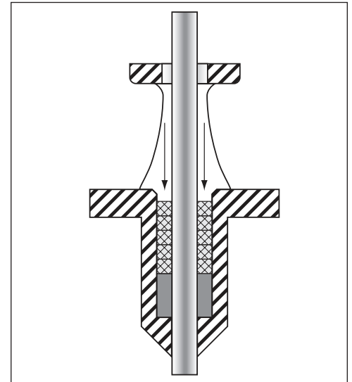
Figure 3: Install Bushing and Packing Rings
