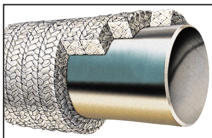
Solution: Chesterton 1730 Mill Pack is resistant to heat and abrasives, will not glaze, unlike common mill packings
