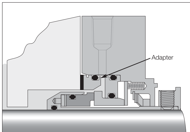
180H Seal Assembly Cross Section
