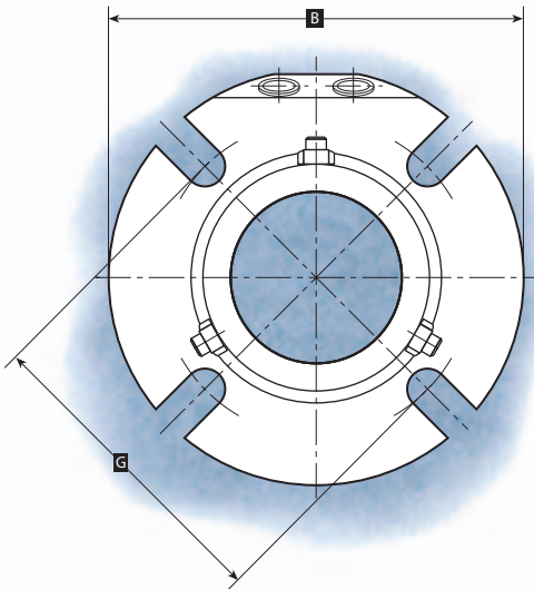
280 MIXER – Dimensional Data/Metric
