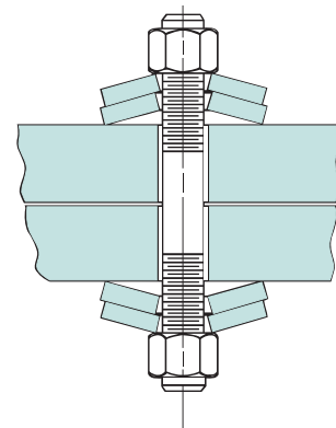
Live Loaded Flange
